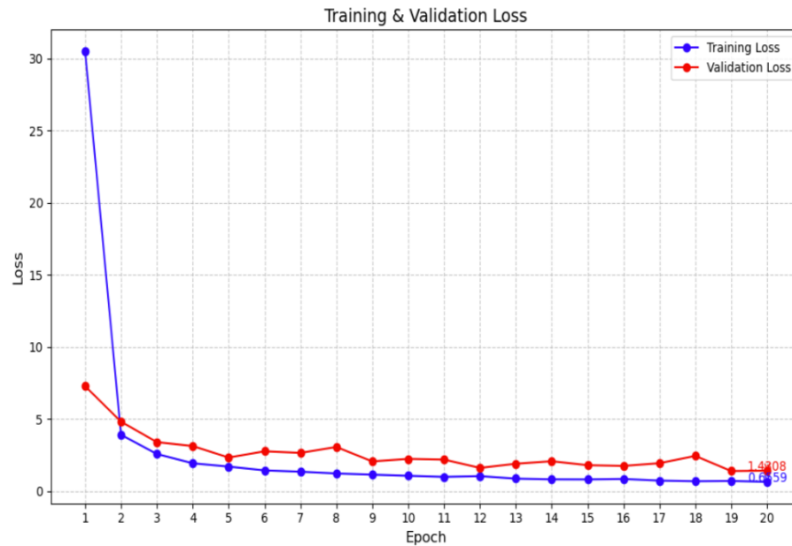
Fig.20. Train and validation loss for ViT model
