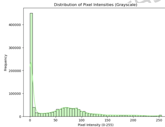
Fig. 8. Distribution of Pixel Intensities Distribution
