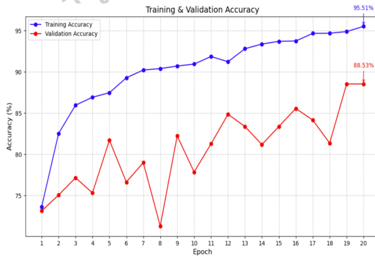
Fig.19. Train and validation accuracy for ViT model
