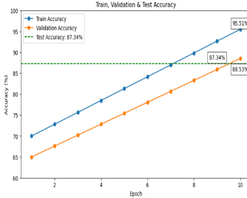
Fig.22. ViT model train, test and validation accuracy
