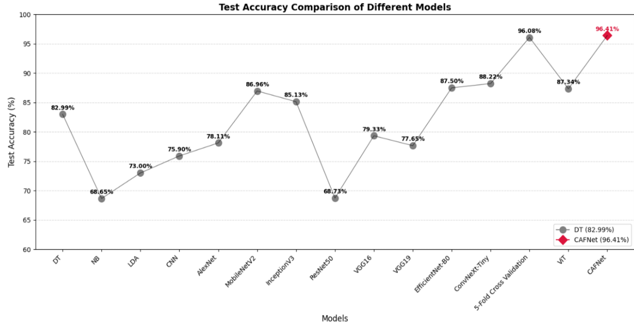
Fig.27. Overall Performance Analysis
