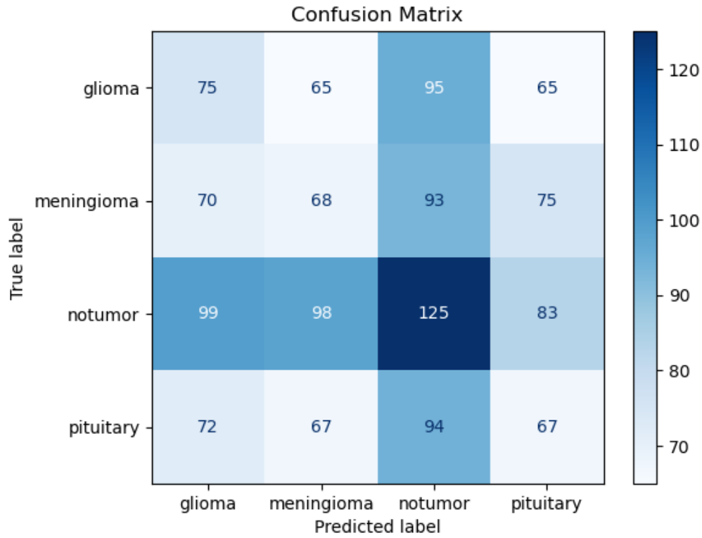
Fig.26. Confusion matrix for CAFNet
