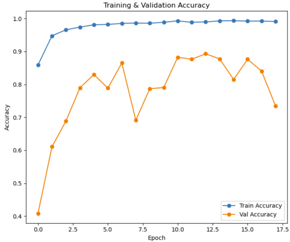
Fig.24. CAFNet Training and Validation Accuracy
