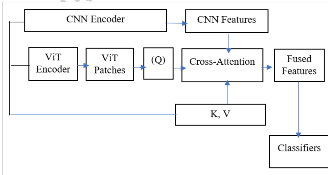
Fig.23. Cross-Attention Fusion (CAF)
