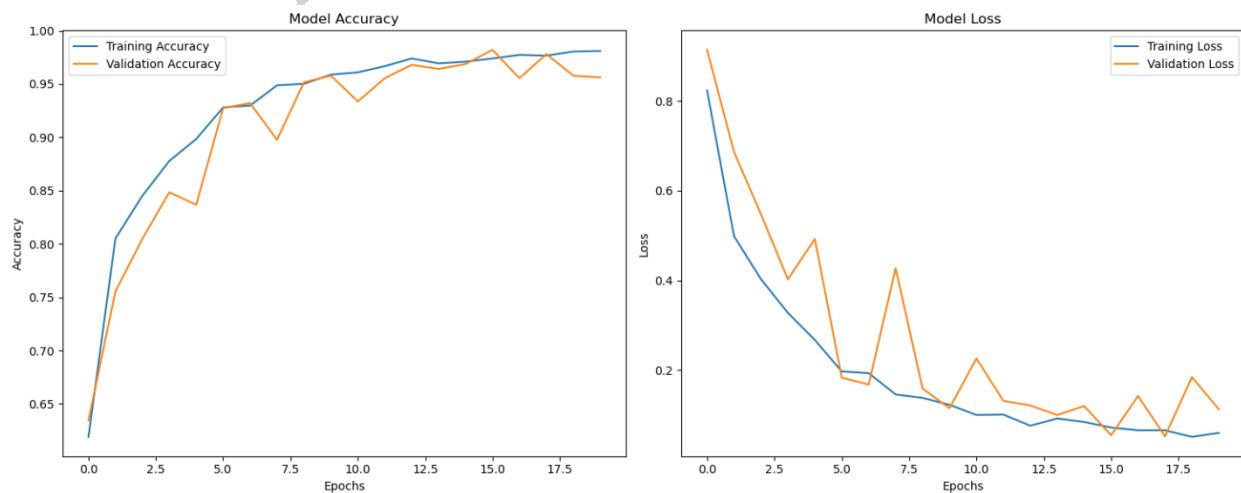
Fig. 13. CNN Model Accuracy and Loss
