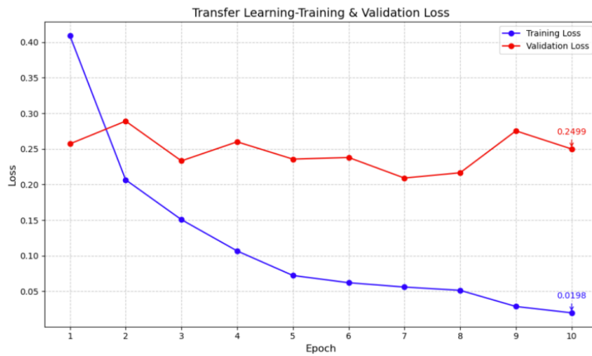
Fig.15. TL models train and validation loss
