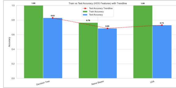
Fig. 9. Standard ML Classifiers Performance Analysis
