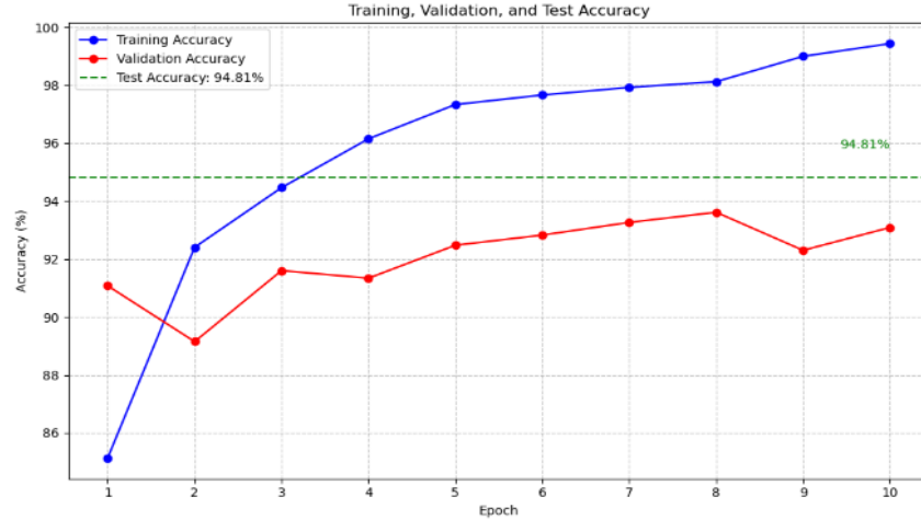
Fig.16. TL models training, testing and validation accuracy
