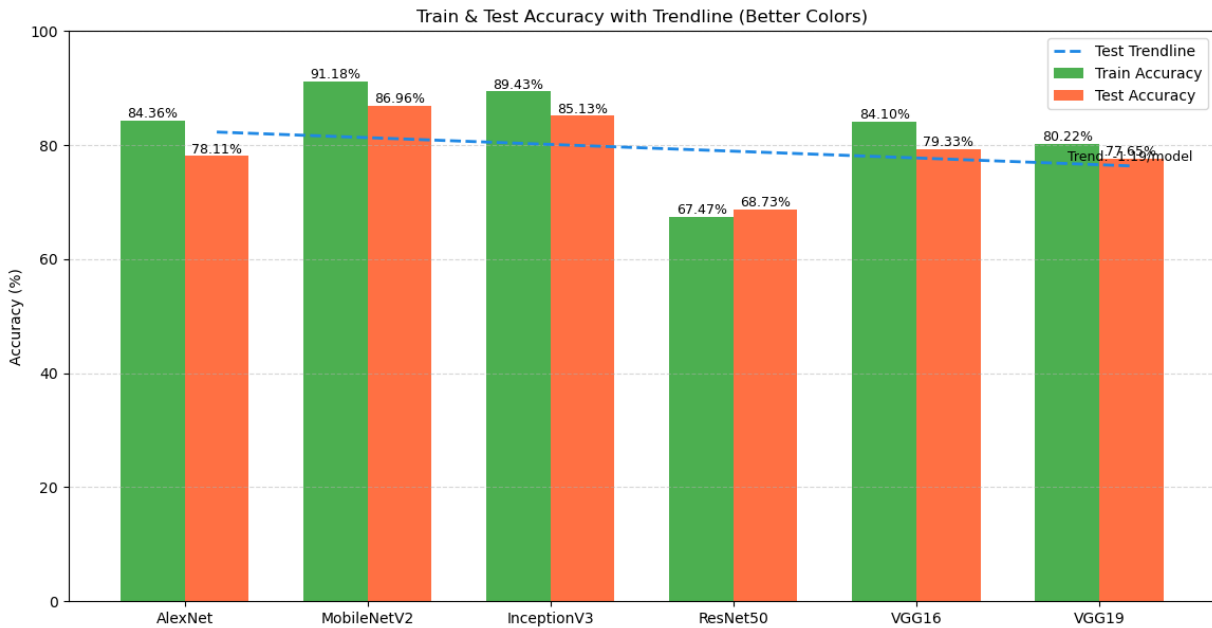
Fig.17. Performance analysis for TL Models
