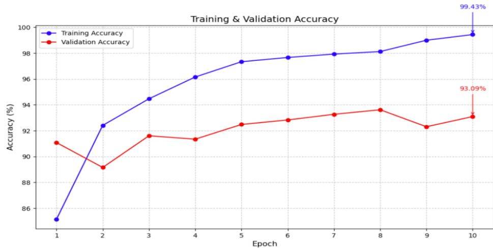
Fig.14. TL models train and validation accuracy
