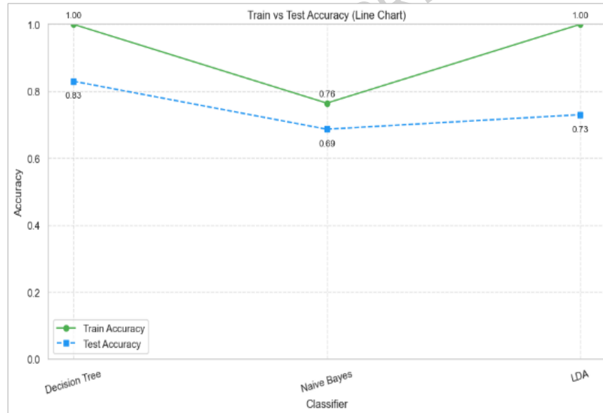
Fig.10. Performance Analysis of DT, NB and LDA.
