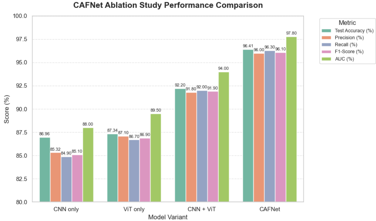
Fig.28. Ablation Study Performance Analysis
