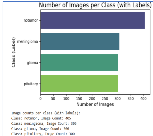
Fig. 3 Test Dataset Class Distribution
