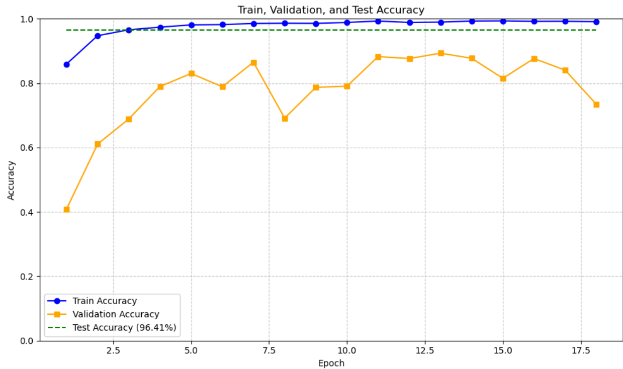
Fig.24. CAFNet Training and Validation Accuracy
